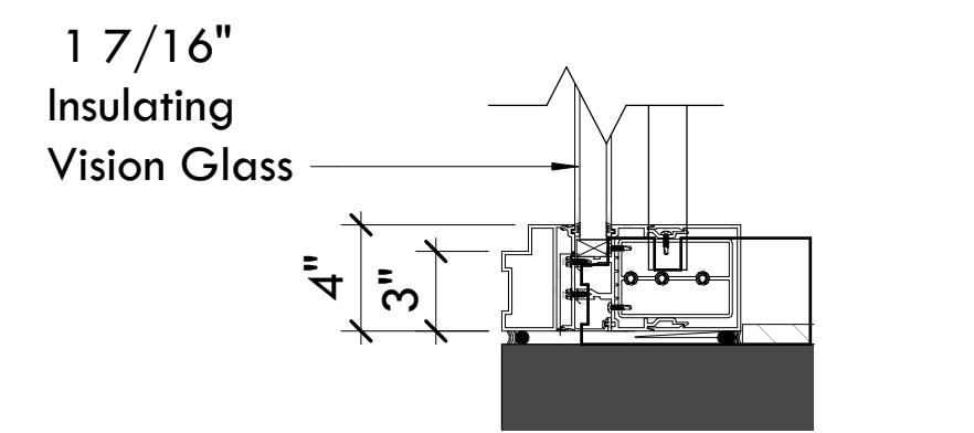
② Window Profile Section 1 1/2" = 1'-0"
