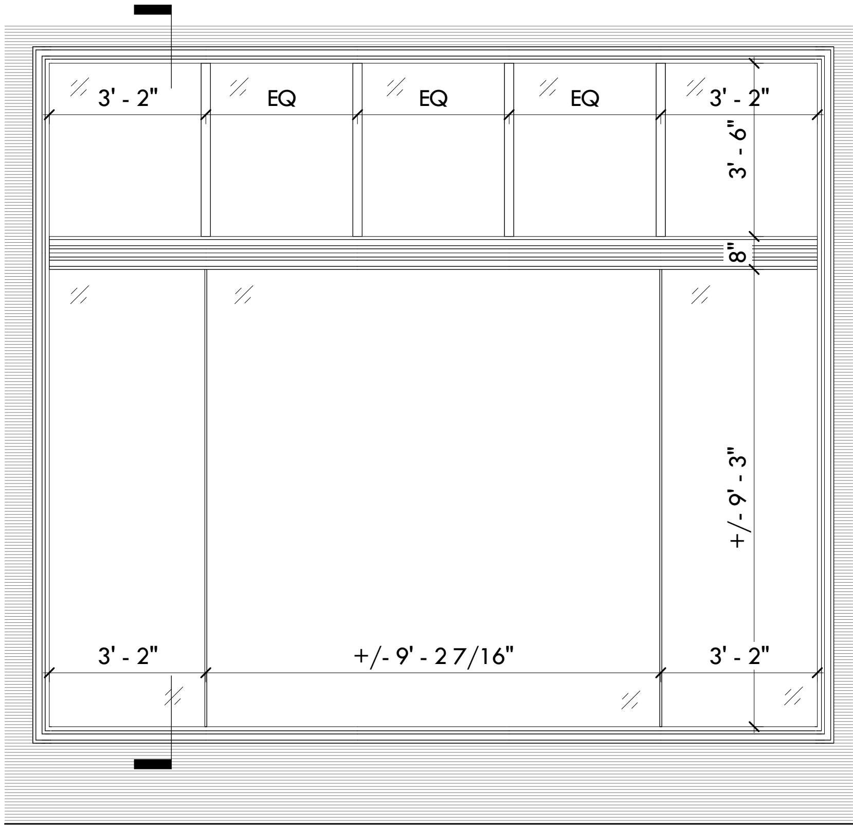
④ Typical 5 Part Storefront System - Planning Commission 1/2" = 1'-0"
