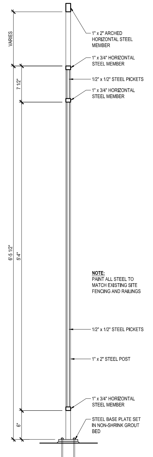
TYPICAL FENCE SECTION
